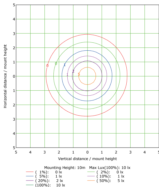
IsoLux Plot
